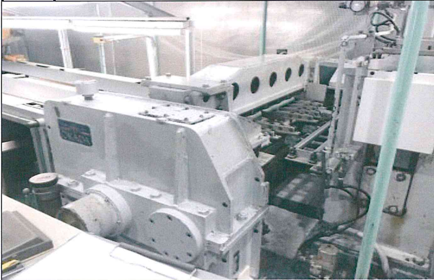
Rotary Shear
